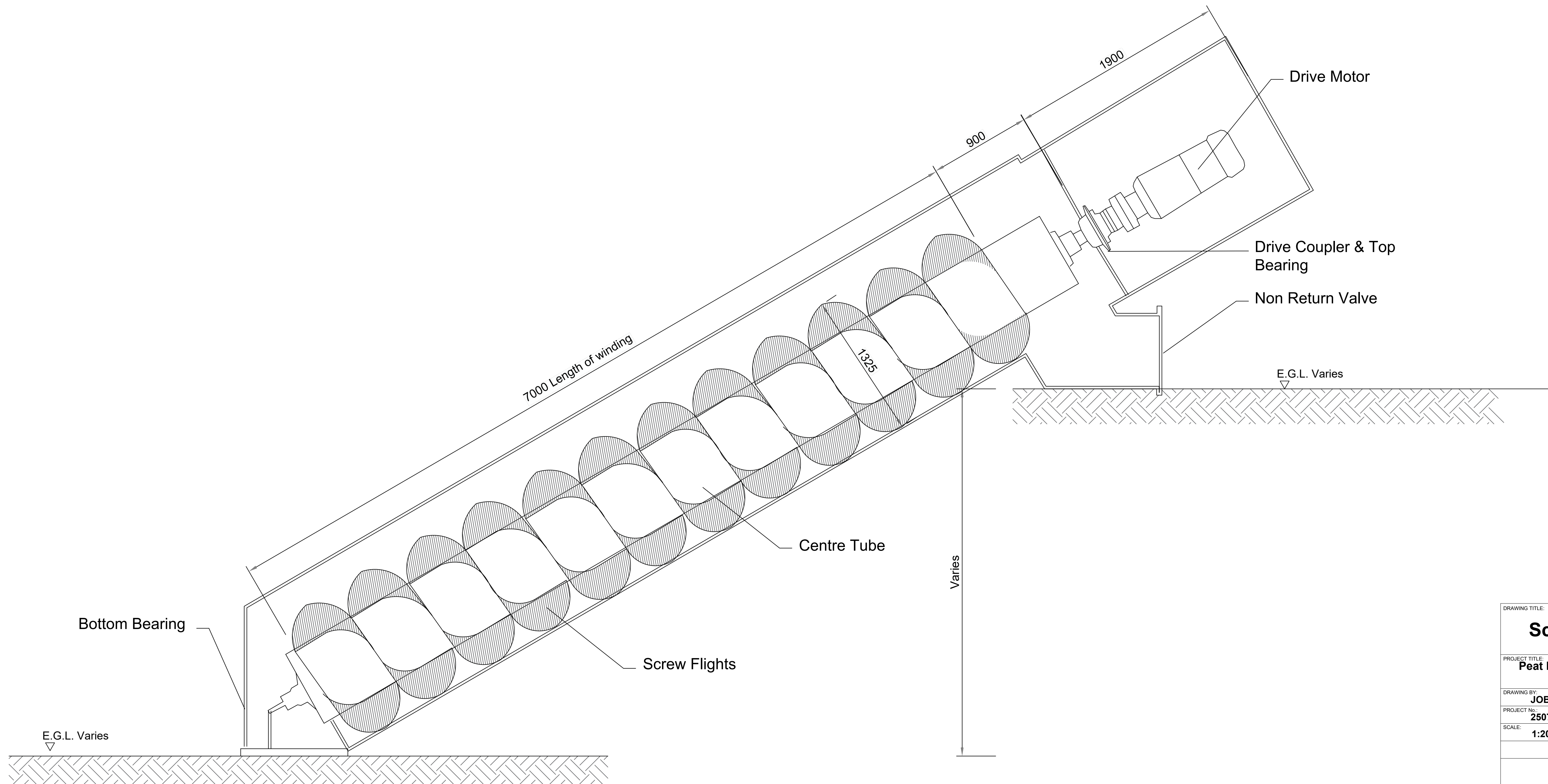
SCREW PUMP - ELEVATION Scale 1:20
